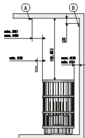
P0 heater's safety distances and the location options for the sensor (A,B)
